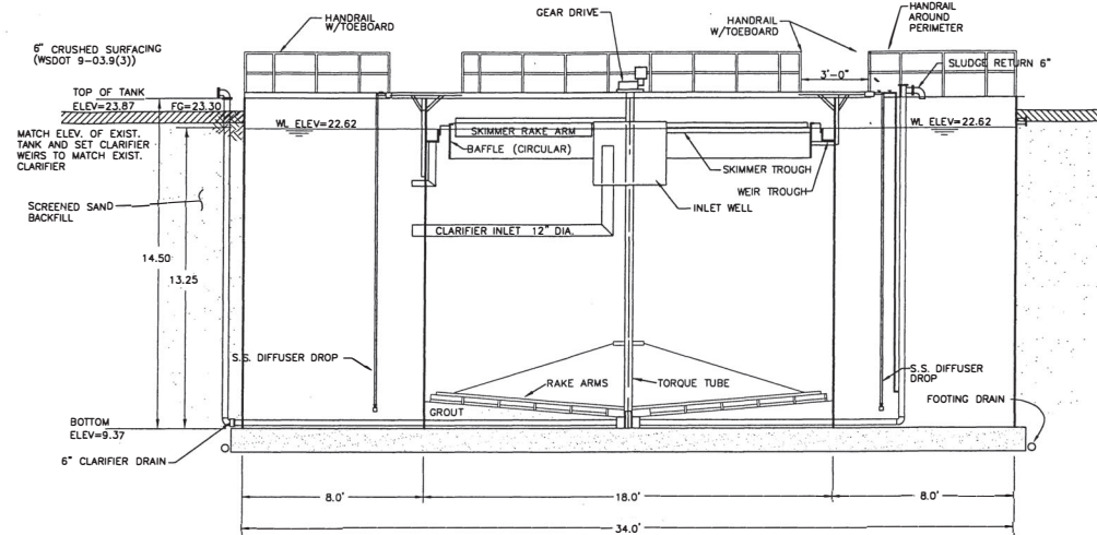
ELEVATION VIEW SCALE: 1"=3'
